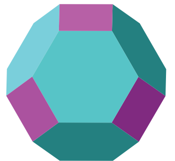
Truncated octahedron
