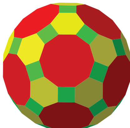
Rhombitruncated icosidodecahedron
