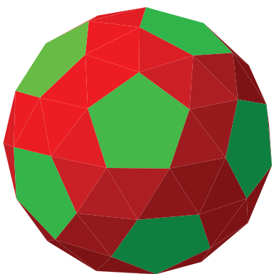
Snub icosidodecahedron
