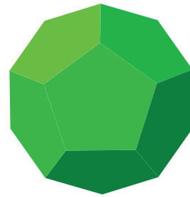
Dodecahedron
