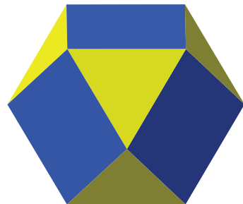
Cuboctahedron
