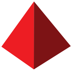
Tetrahedron
