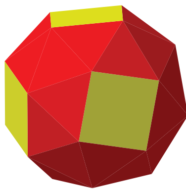
Snub cuboctahedron
