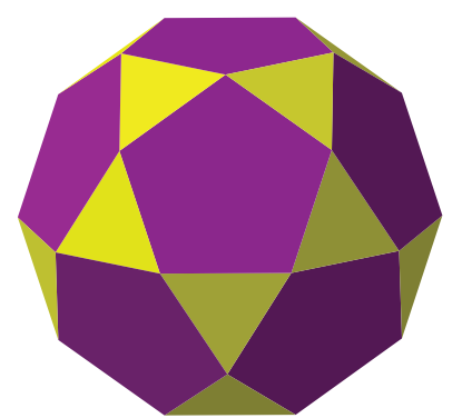
Icosidodecahedron
