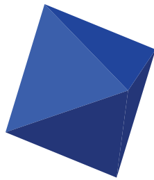
Octahedron
