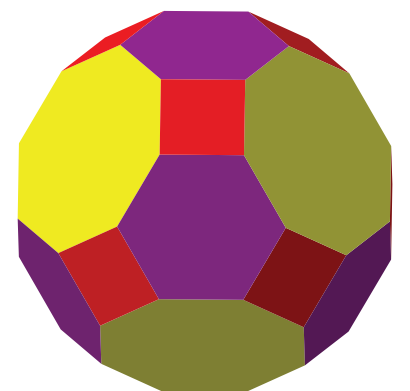
Rhombitruncated cuboctahedron
