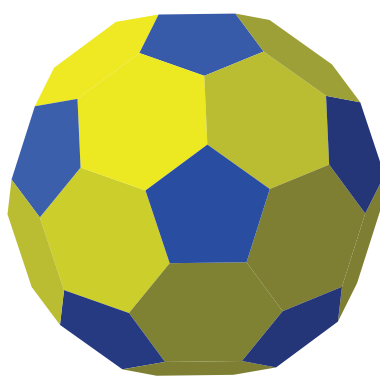
Truncated icosahedron
