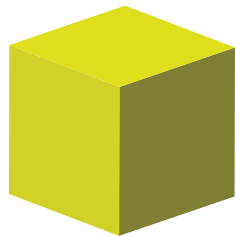
Cube (Hexahedron)
