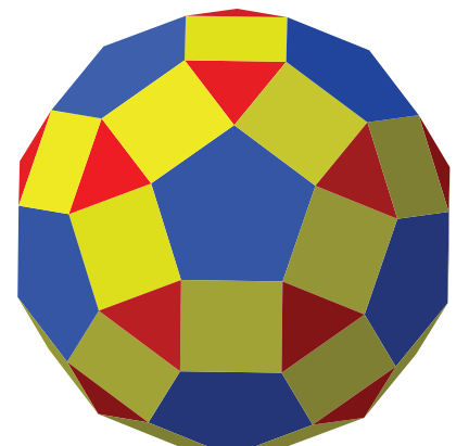
Rhomicosidodecahedron
