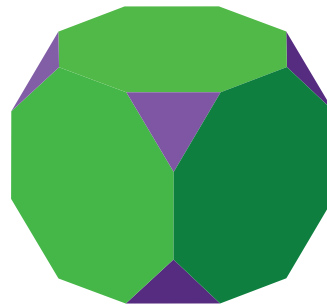
Truncated cube
