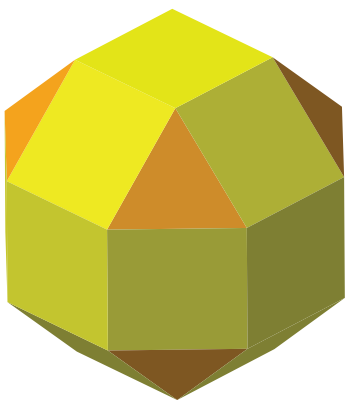
Rhombicuboctahedron
