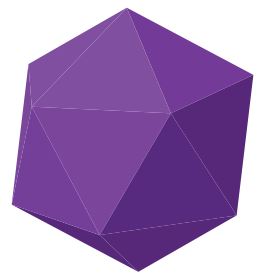
Icosahedron
