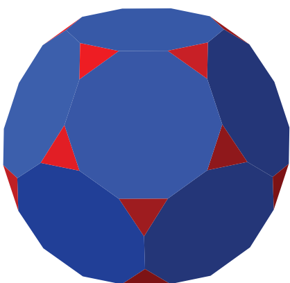
Truncated dodecahedron
